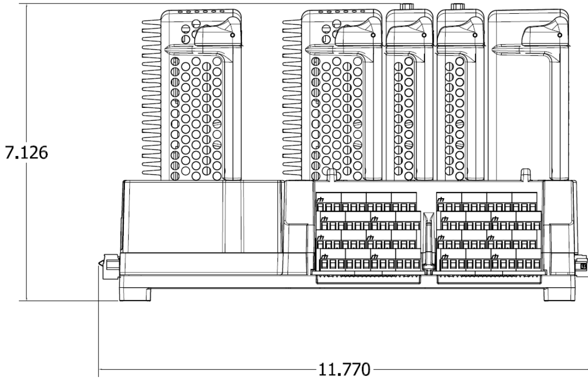
Figure 4: 3701/40 Duplex Terminal Base Side View
