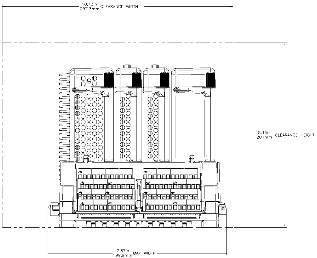
Figure 3: 3701/40 Simplex Terminal Base Side View
